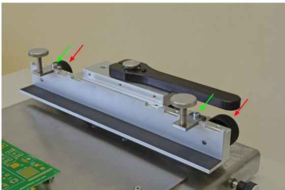
Stencil clamping mounted
